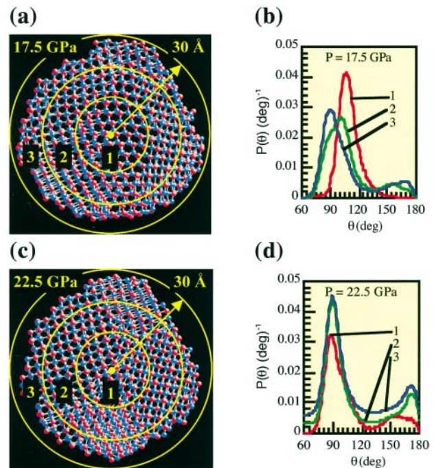
FIG. 2 (color). Structural transformation in a GaAs nanocrystal from outer to inner shells. 8 Å slice of the spherical nanocrystal of diameter 60\text{ \AA} at a pressure of 17.5 GPa (a) and at 22.5 GPa (c). Bond-angle distributions at 17.5 GPa (b) and at 22.5 GPa (d).
