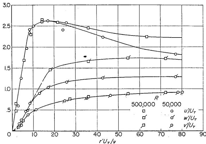
FIGURE 25.— u' , v' , and w' distributions near wall.
