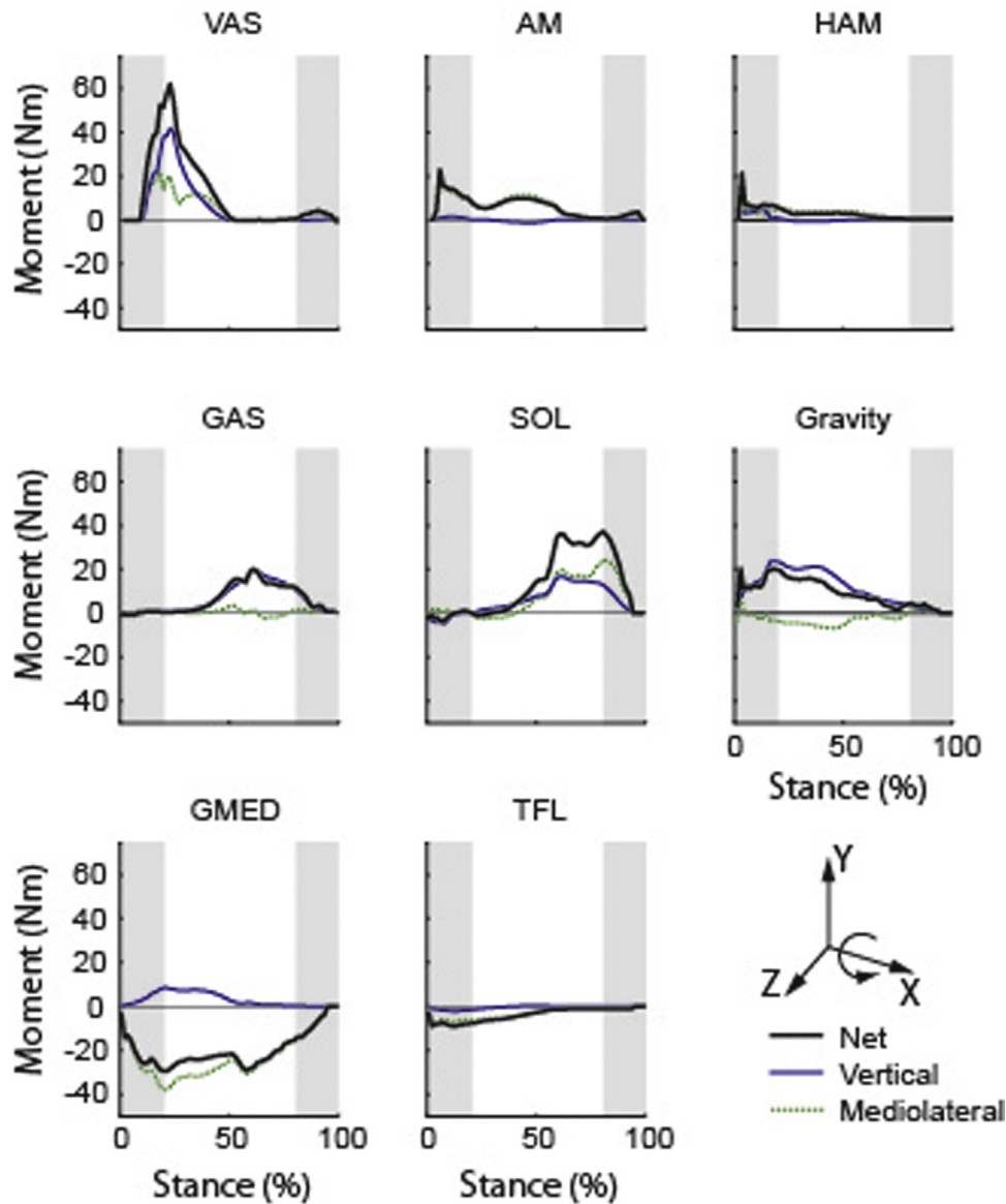
Fig. 3. Individual muscle contributions to the time rate of change of frontal plane angular momentum ( \dot{H} about the x -axis). M/L is the contribution from the mediolateral ground reaction force, Vertical is the contribution from the vertical ground reaction force. Net is the summed contribution from the mediolateral and vertical components. All other muscle contributions were small and not shown. Positive (negative) values indicate the muscle acts to rotate the body towards the contralateral (ipsilateral) leg. Shaded regions indicate timing of the double support phases.
