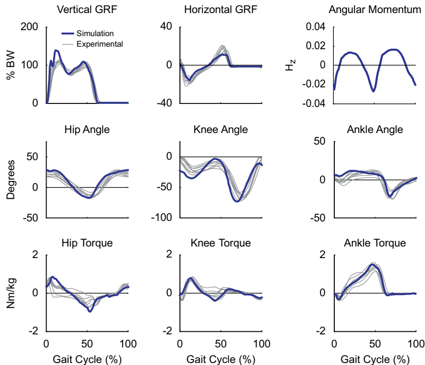
Fig. 2. Comparison between the simulation (thick line) and experimentally collected human subject (thin lines) data (McGowan et al., 2008). Thin lines represent individual averages for each subject's ground reaction forces, joint angles, and intersegmental joint moments. Also shown is the simulation whole-body angular momentum about the medial–lateral axis (Hz) normalized by the product of body mass, height, and walking speed. Due to the marker set used to collect the experimental data, whole-body angular momentum from the subjects could not be computed.
