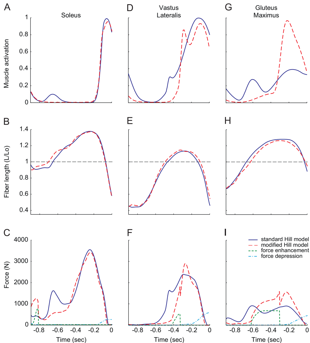
Fig. 6. Simulated muscle data for the soleus, vastus lateralis and gluteus maximus from the control simulation (solid lines) and simulation with the modified-muscle model (dashed lines). Muscle activation patterns (top row) were allowed to vary between the two simulations. Slight differences in kinematics produced small differences in muscle length change (middle row). The magnitude of force generated by muscles with the modified-muscle model included both stretch-induced force enhancement and shortening-induced force depression.
