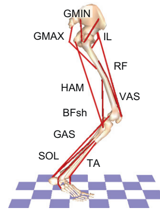
Fig. 4. The musculoskeletal model for simulations of countermovement jumping (right side shown) consisted of rigid segments representing the trunk and two legs, with each leg consisting of a thigh, shank, patella, and three-part foot for a total of 13° of freedom (flexion/extension at the hip, knee, ankle, mid-foot and toes of each leg along with vertical and horizontal translation and rotation of the trunk). The model was driven by 25 musculotendon actuators per leg grouped into 13 muscle groups based on anatomical function: IL (iliacus, psoas), GMAX (gluteus maximus, adductor magnus), GMED (anterior and posterior regions of the gluteus medius), VAS (3-component vastus), RF (rectus femoris), HAM (medial hamstrings, biceps femoris long head), BFsh (biceps femoris short head), GAS (medial and lateral gastrocnemius), SOL (soleus, tibialis posterior), TA (tibialis anterior, peroneus tertius), PR (peroneus longus, peroneus brevis), FLXDG (flexor digitorum longus, flexor hallucis longus) and EXTDG (extensor digitorum longus, extensor hallucis longus). PR, FLXDG, and EXTDG are not shown. Each muscle within a group received the same excitation pattern.
