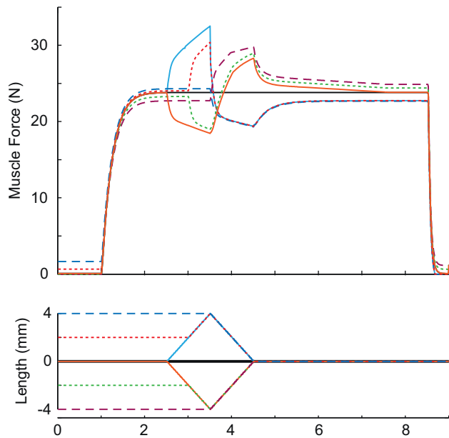
Fig. 3. Simulated force data from the modified muscle model for active stretch-shorten and shorten-stretch cycles. Stretch-shorten cycles consisted of 4 mm contractions preceded by active stretches of 0 mm, 2 mm and 4 mm. Shorten-stretch cycles consisted of 4 mm stretches preceded by contractions of 0 mm, 2 mm and 4 mm. All length changes occurred at 4 mm/s and ended at the muscle's optimal length. The modified muscle model includes both stretch induced force enhancement and shortening induced force depression. Colors and line patterns are the same for muscle force and length for each condition. Consistent with experimental data, history dependent effects are cumulative during shorten-stretch cycles but not during stretch-shorten cycles.
