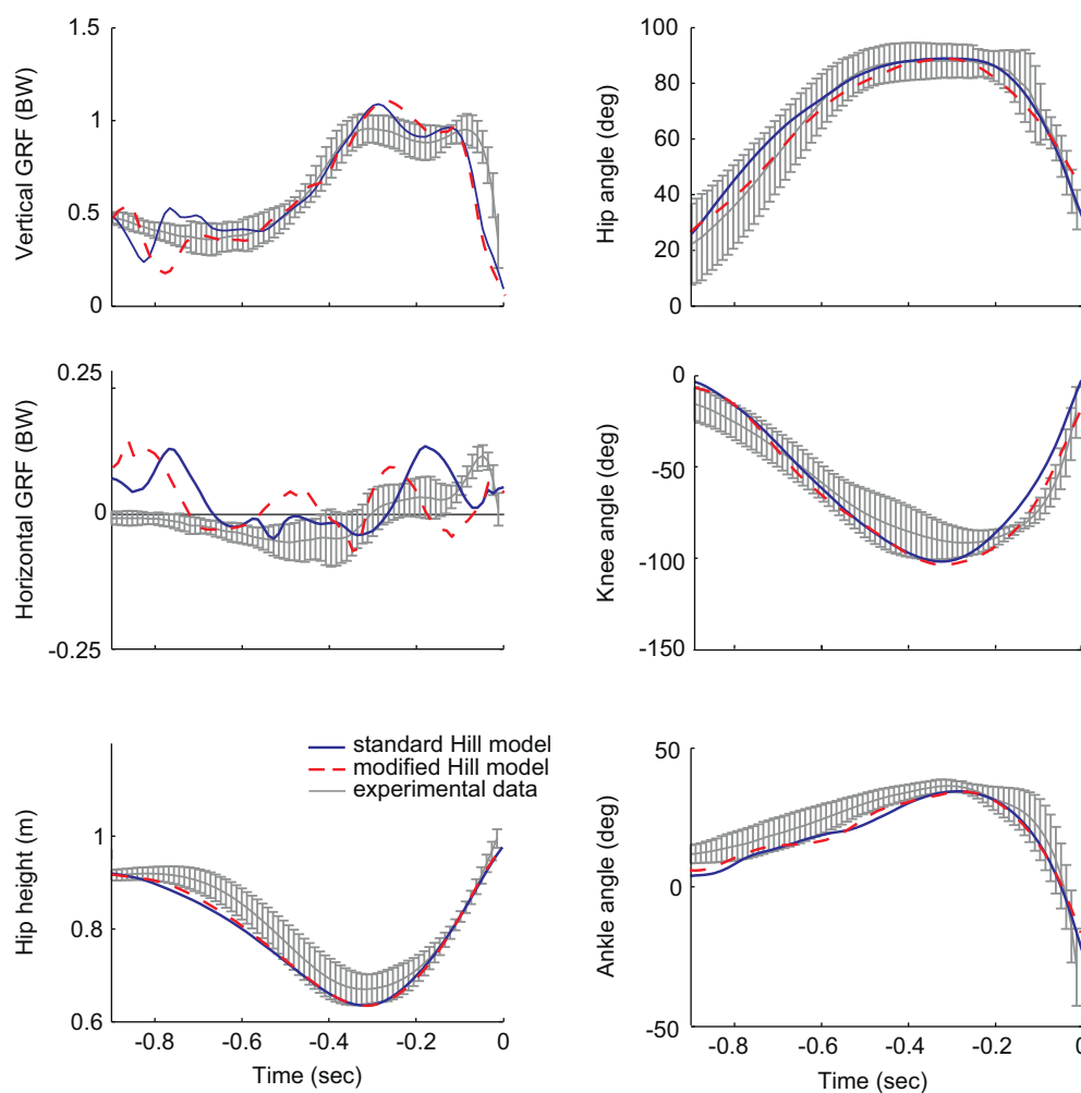
Fig. 5. Ground reaction force and kinematic data from the counter movement jump. The gray lines are the average experimental data ( \pm 2 standard deviations) from 10 jumping trials from a single subject. The solid blue lines are data from the control simulation and the dashed red lines are data from simulation with the modified muscle model. (For interpretation of the references to color in this figure legend, the reader is referred to the web version of this article.)
