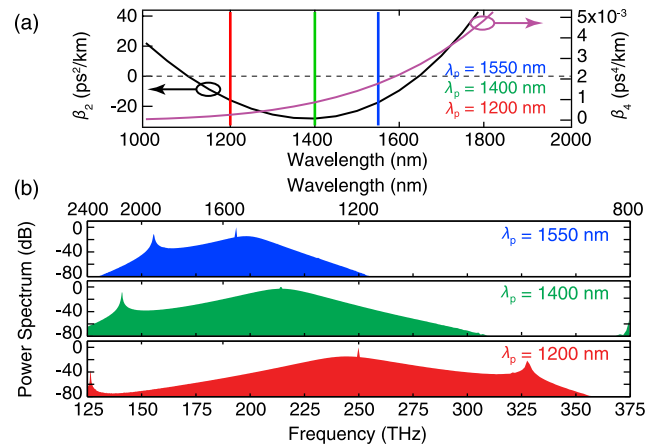
Fig. 2. (a) Simulated GVD and FOD for 690 \times 1900 nm cross section \text{Si}_3\text{N}_4 waveguide. (b) Simulated comb spectra for pump wavelengths of 1550 , 1400 , and 1200 nm.
