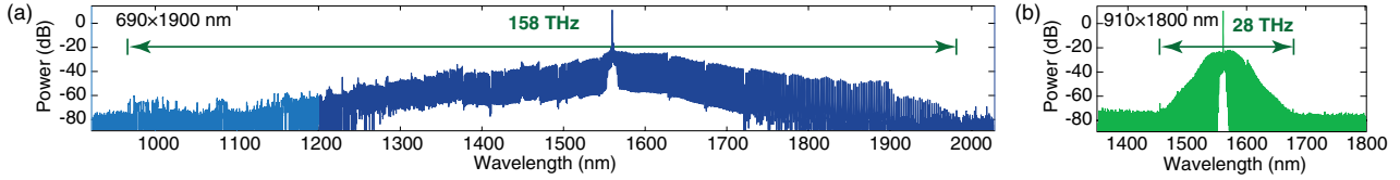
Fig. 3. Measured comb spectra in \text{Si}_3\text{N}_4 microrings with cross sections (a) 690 \times 1900 nm and (b) 910 \times 1800 nm.
