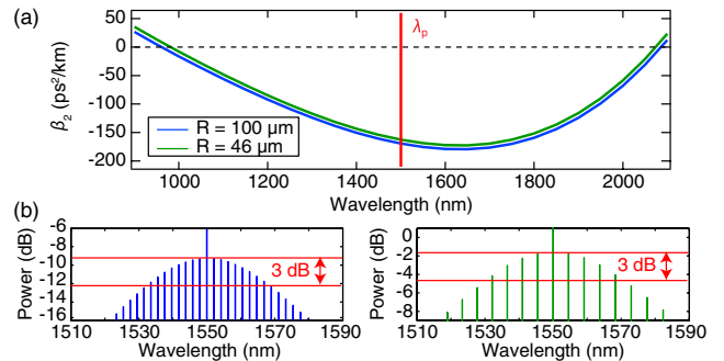
Fig. 4. (a) Simulated GVD for 950 \times 1400 nm cross section \text{Si}_3\text{N}_4 microrings for a 100 and 46 \mu\text{m} radius. (b) Simulated comb spectra in 100 and 46 \mu\text{m} radius microrings, corresponding to 260 and 530 GHz FSRs, respectively.
