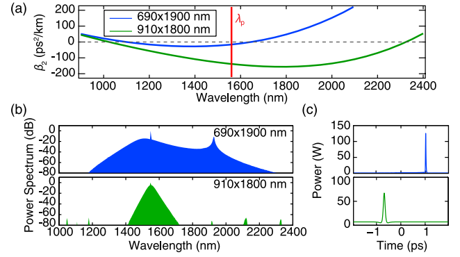
Fig. 1. (a) Simulated GVD for silicon-nitride waveguides with cross sections 690 \times 1900 nm (blue) and 910 \times 1800 nm (green). (b) Simulated comb spectra and (c) temporal plot for 260 GHz free spectral range (FSR) \text{Si}_3\text{N}_4 microring resonators with cross sections 690 \times 1900 nm (top) and 910 \times 1800 nm (bottom).
