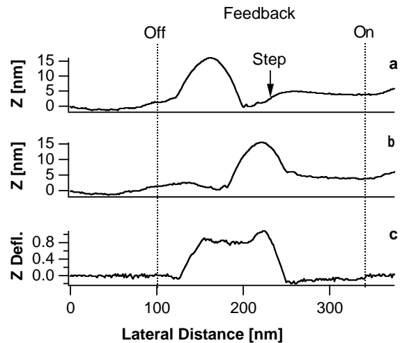
Figure 4. Pushing a particle against a step. Topography signal (a) before and (b) after pushing, and (c) cantilever deflection during pushing.
