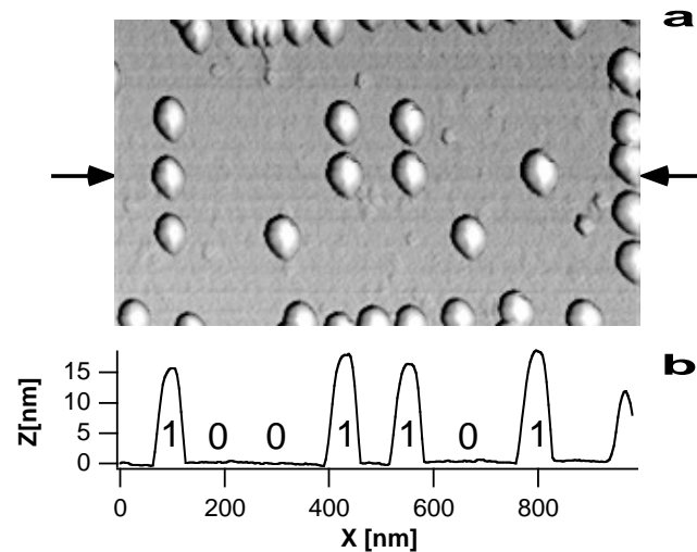
Figure 1. (a) The characters ‘LMR’ ASCII-encoded in rows of nanobits, and (b) the trace obtained by reading the second row with an AFM.
