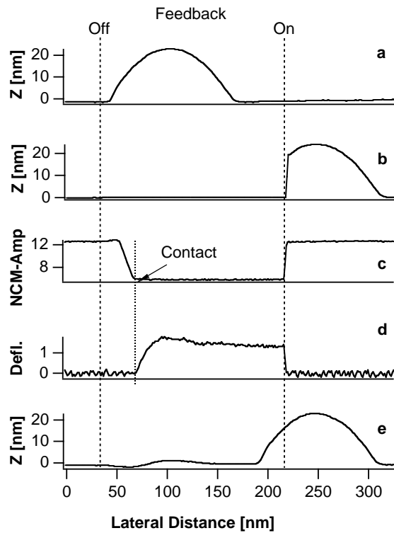
Figure 2. Data associated with a pushing event, as explained in the text. The vertical broken lines denote the points where the feedback is turned off and on.
